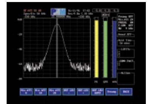
Typical Fundamental Spectral Purity measured with PMM 9000 Receiver
