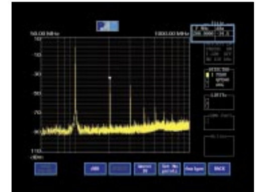
Typical Output Spectral Purity measured with PMM 9000 Receiver
